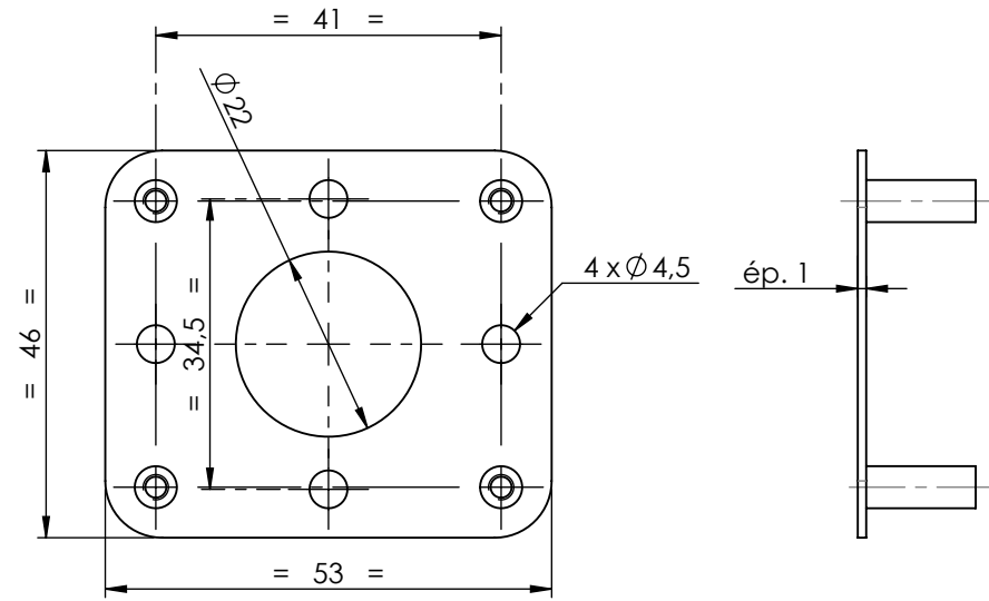
Support inox de fixation
